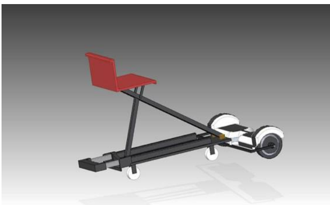
Figure 4: Side View of Segwalk 11.
