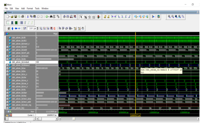
Figure 6: DDR SDRAM memory controller design wave form.
