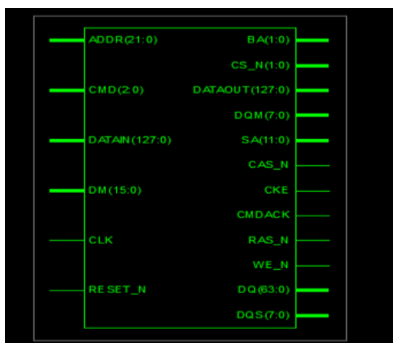
Figure 2: RTL schematic of DDR Controller
