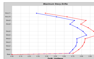
Fig 9.13 Storey Drift at zone 2 by Static Analysis
