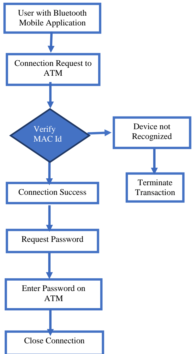
Fig 7.2.2: Wireless Password Transfer
