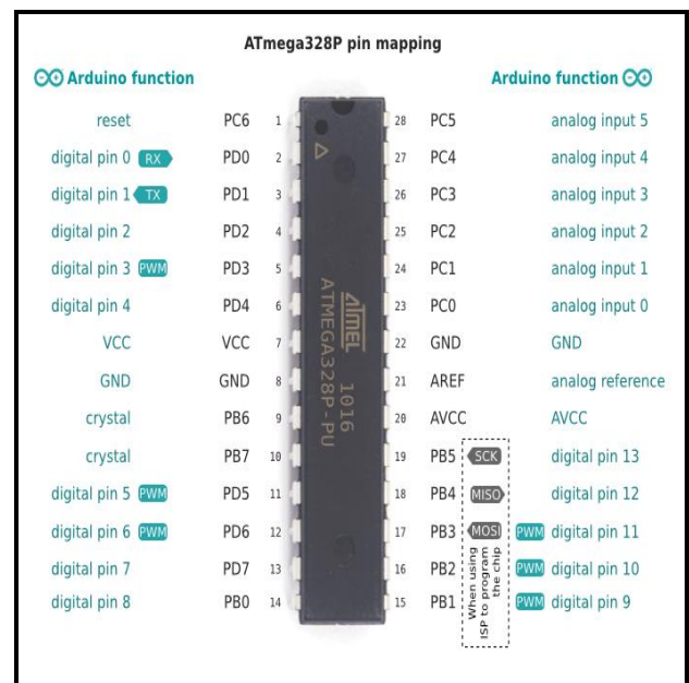
Fig -1: Pin Diagram of Arduino Uno ATmega328P
