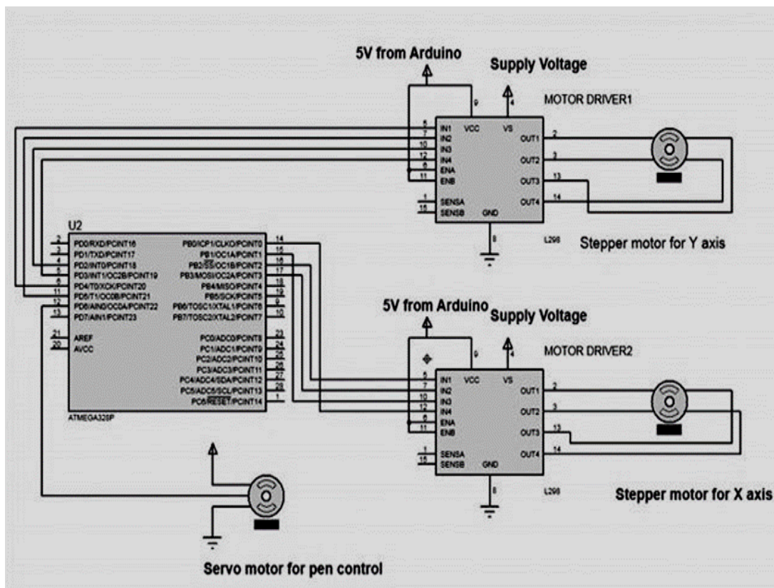
Fig -6: Experimental Circuit Diagram
