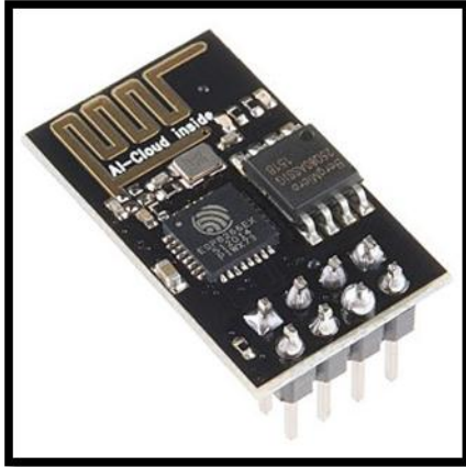
Fig 5 – ESP8266 WIFI Module
