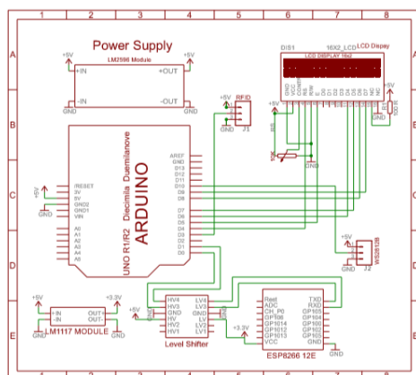
Fig 3 - Schematic Diagram of the connections
