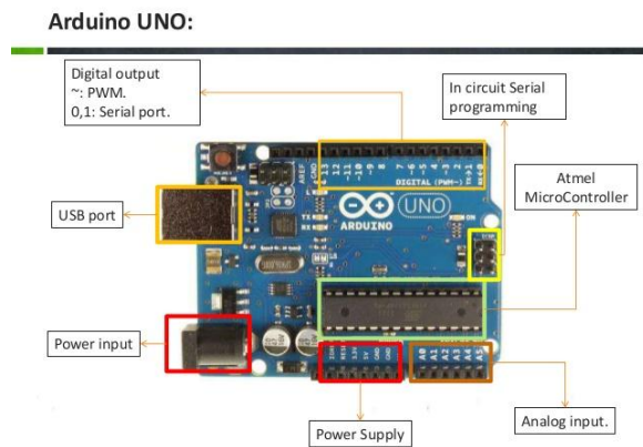
Fig 4 - Arduino Physical Layout
