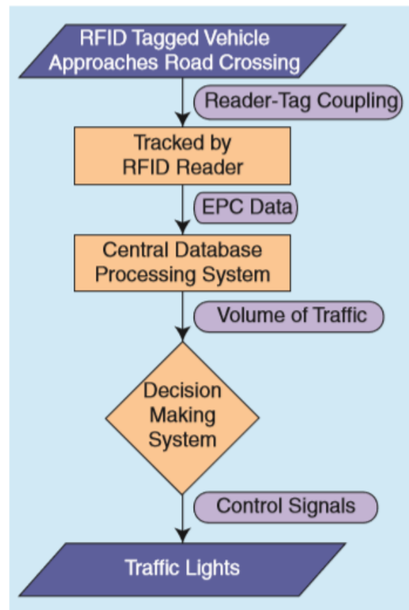
Fig 1. - Flow Chart of sequence of working
