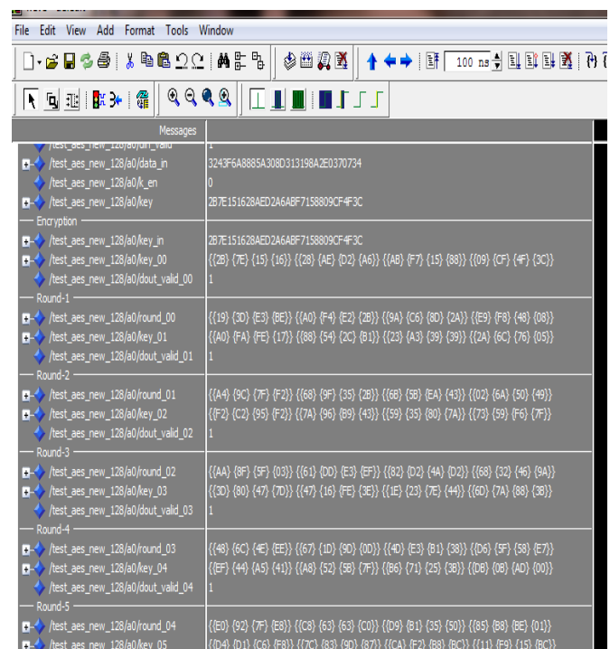
Fig 2.1 encrypted data from round 1 to round 5
