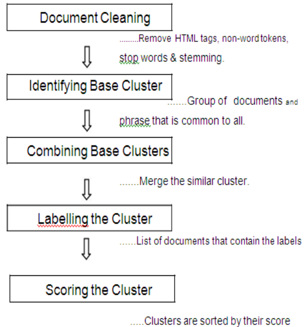
Figure 4. Schematic diagram of Suffix Tree Clustering
