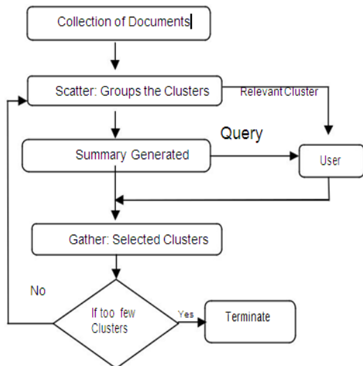
Figure 3. Schematic diagram of Scatter/Gather Clustering Algorithm
