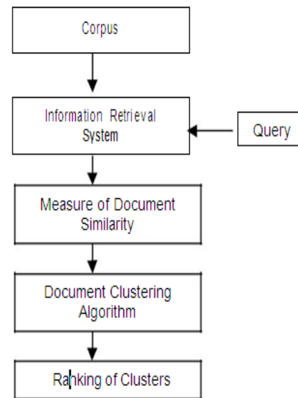
Figure.1 Information Retrieval Framework overview
