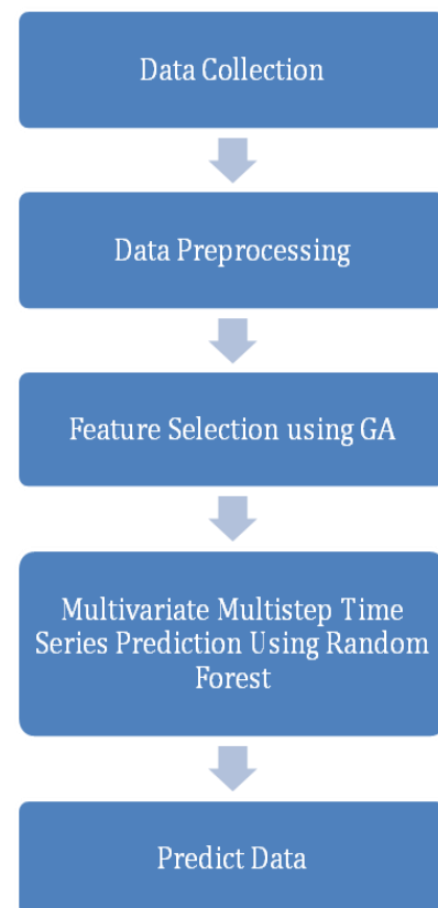
Fig-4: Workflow of proposed method for Air Pollution Prediction
