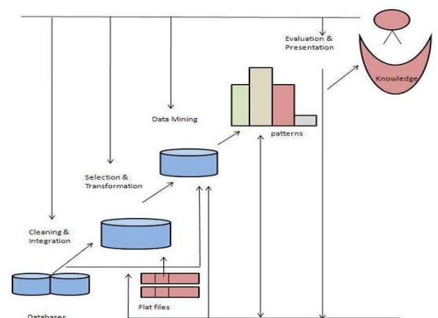
Fig-2: Basic flow diagram of Data Mining for knowledge discovery
