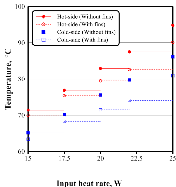
Figure 9. Influence of using fins on the temperature of both sides
