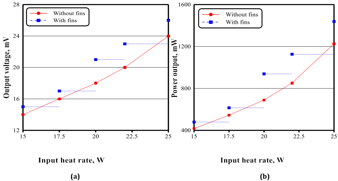
Figure 10. Influence of using fins on the output voltage and power output (a) Variation in the output voltage with input heating rate, (b) Variation in the power output with input heating rate
