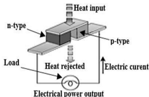
Figure 1. Schematic diagram of a single thermoelectric couple (Thermocouple) [6]
