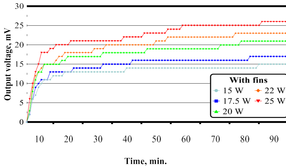
Figure 6. Influence of heating rate on the variation in the output voltage with time, in case of FC (a) Variation in the output voltage with time for various input heating rates, in case of FC without the assist of fins, (b) Variation in the voltage output with time for various input heating rates, in case of FC with the assist of fins.
