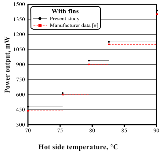
Figure 4. Comparison between the experimental results of the current study and that after reference [18], for the variation in the power output with hot-side temperature
