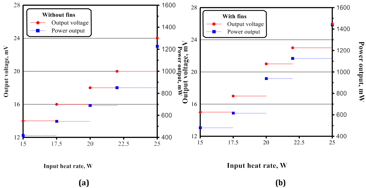
Figure 8. Influence of input heating rate on the output voltage and power output (a) Variation in the output voltage and power output with input heating rate, without fins, (b) Variation in the output voltage and power output with input heating rate, with fins.
