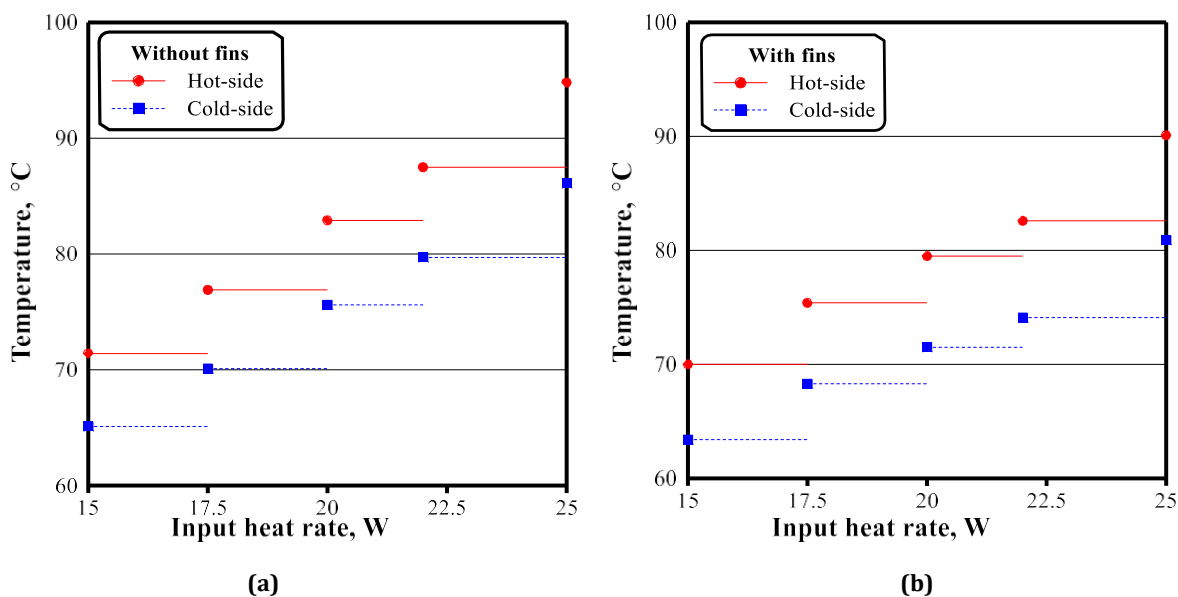
Figure 7. Influence of input heating rate on the temperature of both sides (a) Variation in the temperature of both sides with input heating rate, without fins, (b) Variation in the temperature of both sides with input heating rate, with fins
