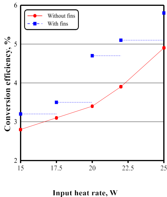
Figure 11. Influence of using fins on the conversion efficiency
