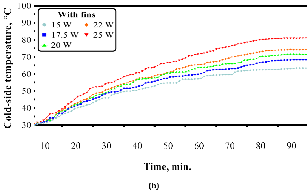
Figure 5. Influence of heating rate on the variation in the temperature of both sides with time, in case of FC
