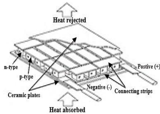
Figure 2. Cut-away view of a typical TEG module [6]
