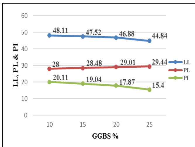
Fig 1 Variations in Consistency Limits of mix having 1% of Sodium Sulphate with various proportions of GGBS.
