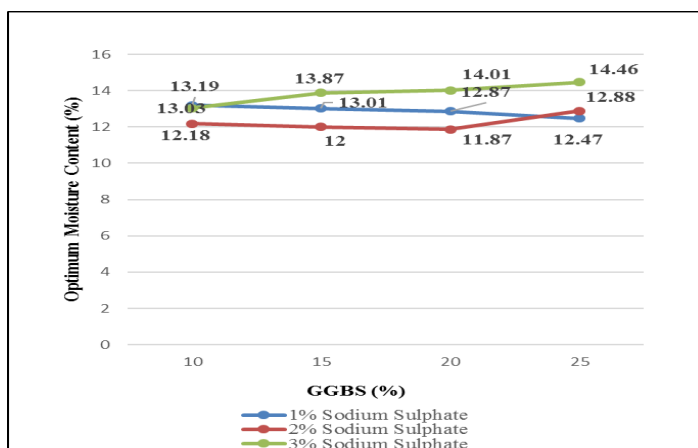
Fig 4 OMC v/s percentage of GGBS with 1%, 2%, 3% of Sodium Sulphate with different proportions of Soil.
