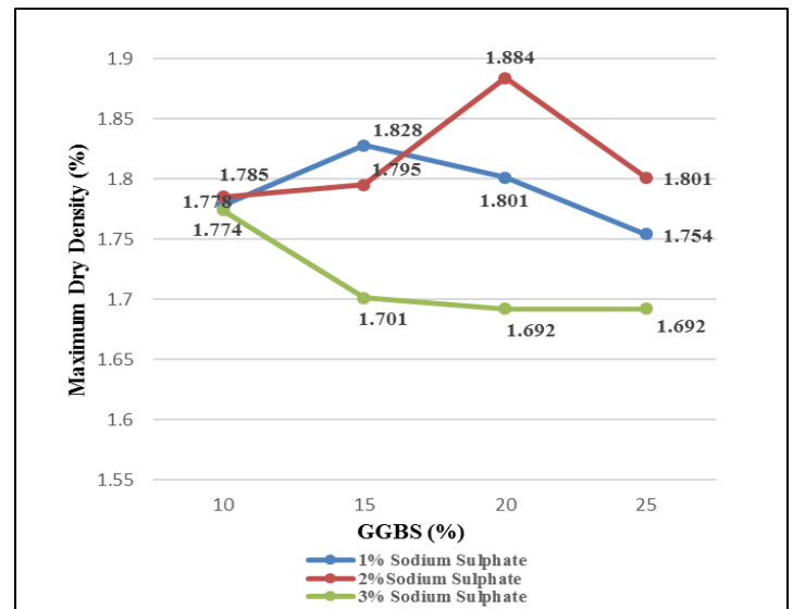
Fig 5 MDD v/s %age of GGBS with 1%, 2%, 3% of GGBS and 1%, 2%, 3% of Sodium Sulphate with different proportions of Soil.
