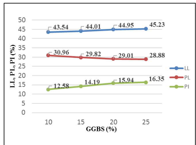
Fig 3 Variations in Consistency Limits of mix having 3% of Sodium Sulphate with various percentages of GGBS.
