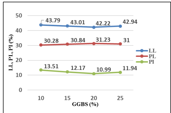
Fig 2 Variations in Consistency limits of mix having 2% of Sodium sulphate with various percentages of GGBS
