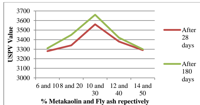
Fig 1.2 USPV test of concrete at the age of 28 days and 180 days
