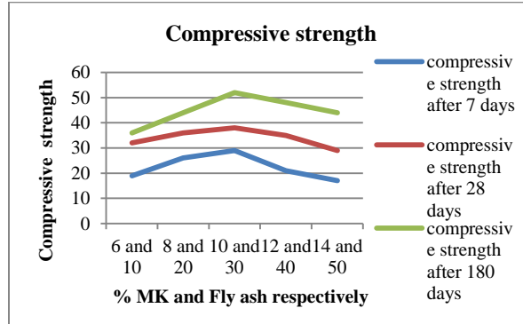
Fig. 1.4 Compressive strength of modified concrete after 7, 28 and 180 days, respectively
