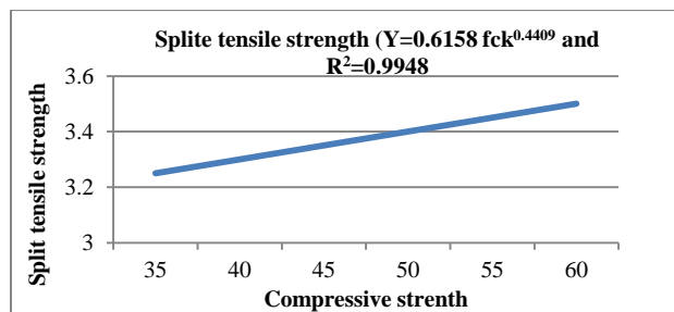
Fig 1.7 Relation between compressive strength and split tensile strength
