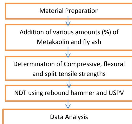
Fig.1 Experimental Flowchart diagram
