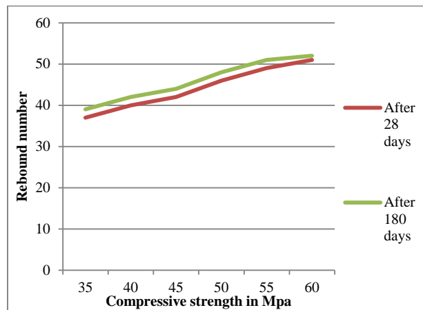
Fig 1.1 Relation between rebound number and compressive strength
