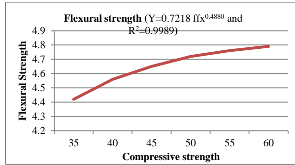
Fig 1.8 Relation between compressive strength and Flexural strength
