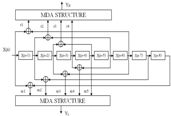
Figure 2: Block Diagram of 9/7 Wavelet Coefficient based Discrete Wavelet Transform
