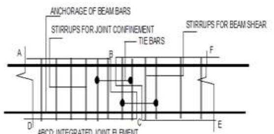
DUCTILE DETAILING OF JOINT ELEMENT (ABCD) & BEAM ELEMENT (BCEF) (CONNECTION DETAILS OF JOINT ELEMENT 4)
