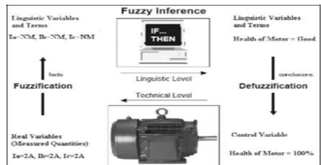
Fig. 3: Motor and fuzzy interface
