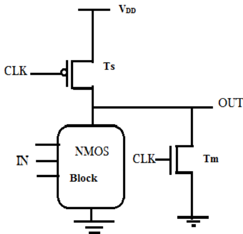
Figure 1: Feed through logic [9]
