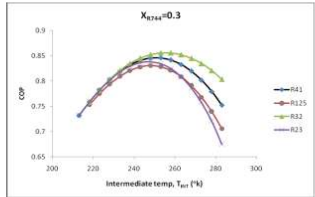
Fig -10: Variation in COP with intermediate temperature for cascade system operating with R744 blend at 0.3 mole fraction as low temperature working fluid with approach 5°C.
