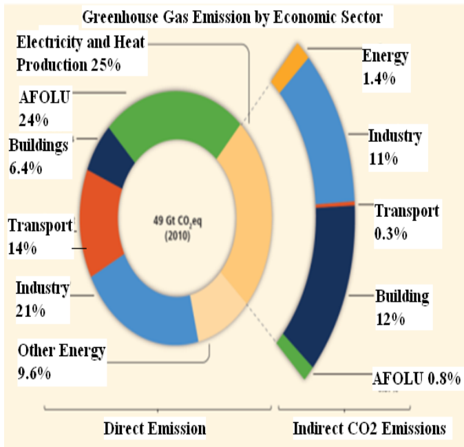
Fig. 1. Carbon Emissions
