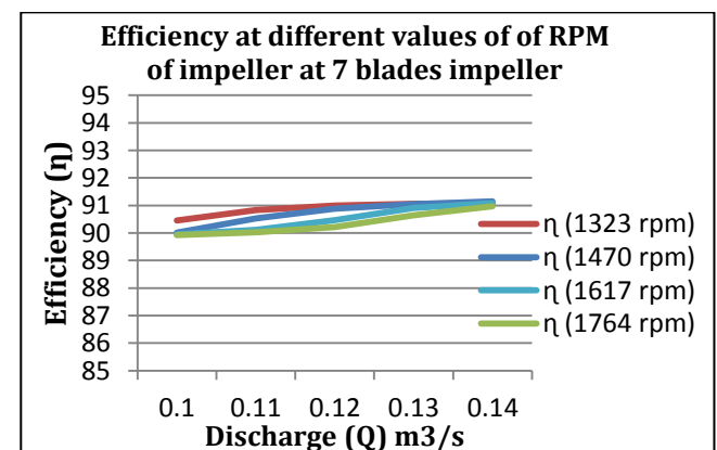
Graph 4.6: Efficiency of pump impeller at different rpm of impeller have 7 number of blades.
