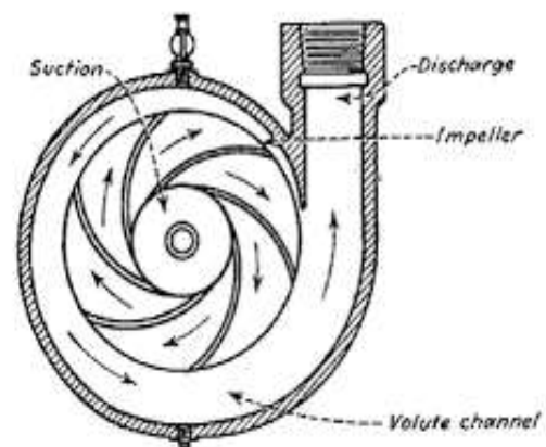
Figure 1.1: Centrifugal Pump.
