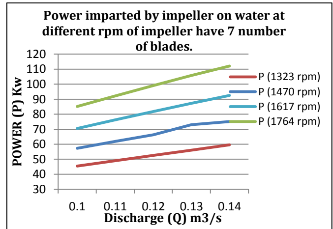
Graph 4.5: Power imparted by impeller on water at different rpm of impeller have 7 number of blades.
