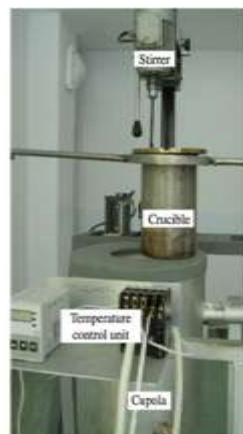
Figure.12 Specimen preparation
