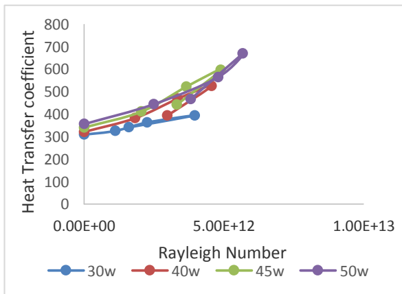
Chart-4: Variation of heat transfer coefficient with Rayleigh number for different heat inputs
