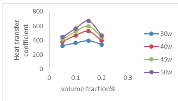
Chart-6: Various heat transfer coefficient with volume fraction of nano fluid for a different heat inputs
