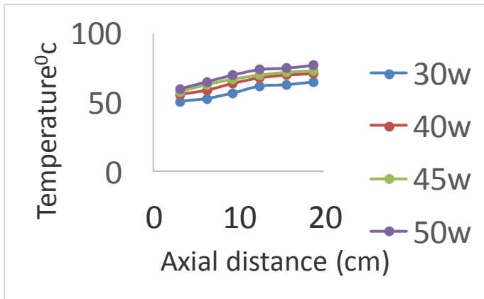
Chart -1: Surface temperature of vertical cylinder along axial direction for transformer oil –TiO 2 at 0.15 vol%
