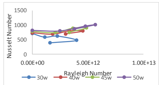
Chart-3: Variation of Nusselt number with Rayleigh number for various heat inputs
