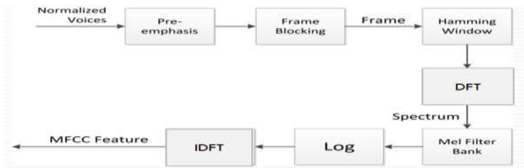
Figure 2: Block diagram of MFCC
