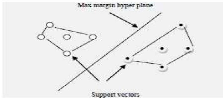
Figure 3: Maximum margin plane and support vectors
