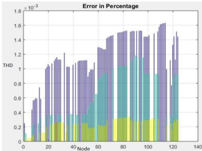
Figure 5. 3 RESULTS OF THD FOR IEEE 123 TEST BUS
