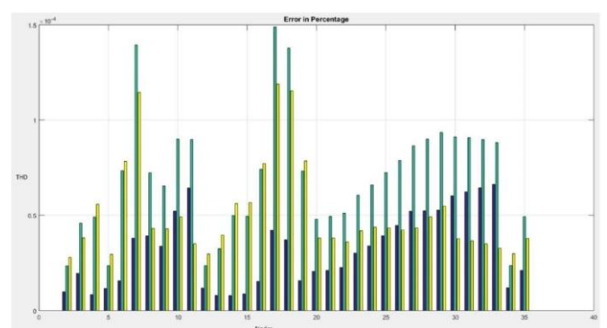
Figure 5. 2 RESULTS OF THD FOR IEEE 37 TEST BUS
