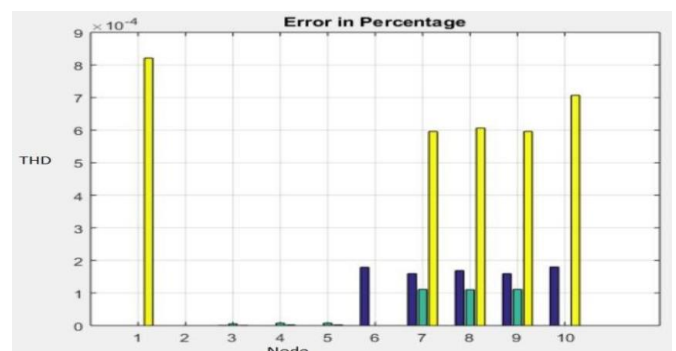
Figure 5. 1 RESULTS OF THD FOR IEEE 13 TEST BUS
