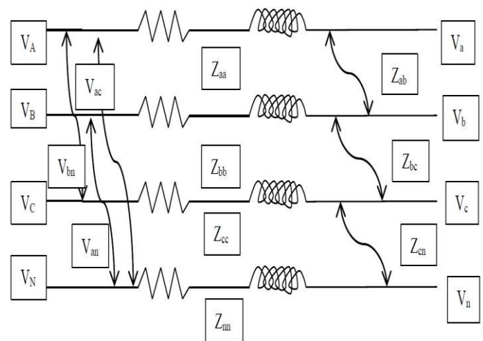
Fig. 3.1 Three Phase Line Section Model
