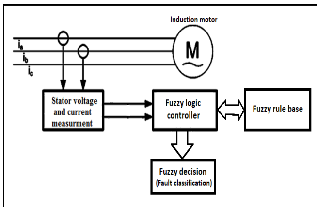
Fig-2: Generalized block diagram of fuzzy logic controller based approach
