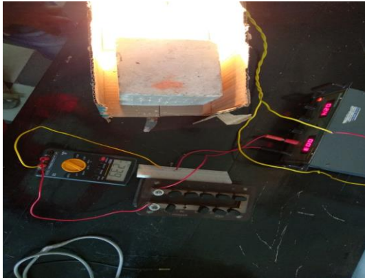
Fig [16] Experimental setup of light transmittance test
