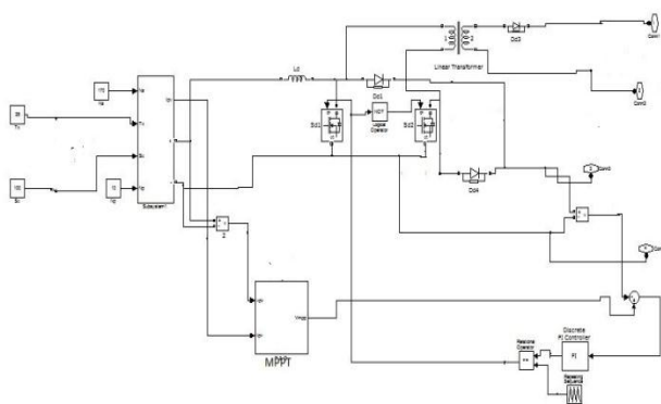
Fig. 6 Matlab simulation of dc-dc converter with PV module and MPPT
