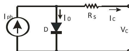
Fig.1 -Equivalent circuit of a PV cell
