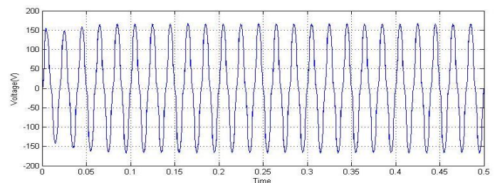
Fig. 9 Output voltage of proposed topology inverter after connecting LC filter.
