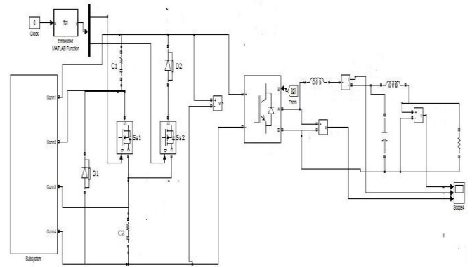
Fig 7 Simulation diagram of seven level inverter
