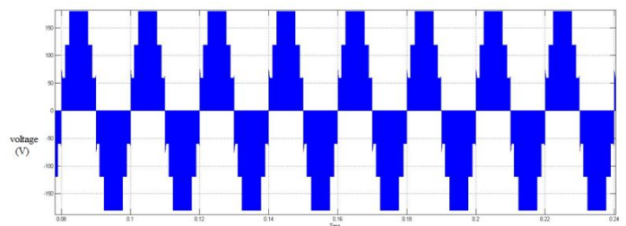
Fig. 8 Seven level output voltage of proposed topology inverter.
