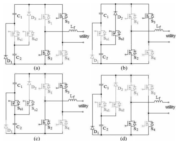
Fig. 4 Operation of the seven-level inverter in the negative half cycle: (a) mode 5, (b) mode 6, (c) mode 7, and (d) mode 8.
