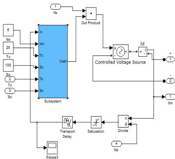
Fig 5 Matlab simulation model of PV cell
