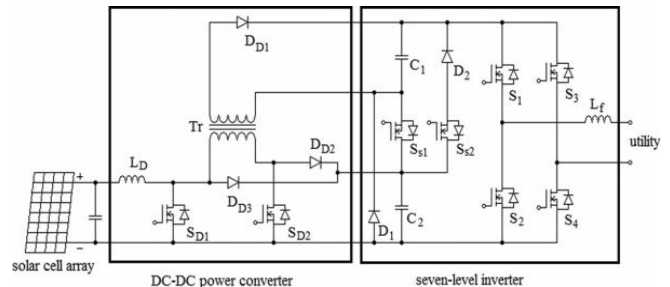
Fig. 2 Proposed solar power generation system
