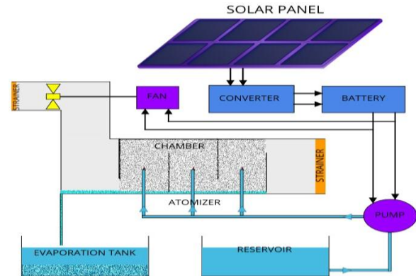
Figure 9: Schematic Diagram
