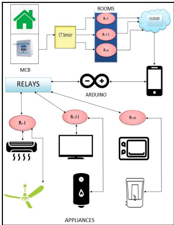
Fig -4: The Architecture of the proposed system
