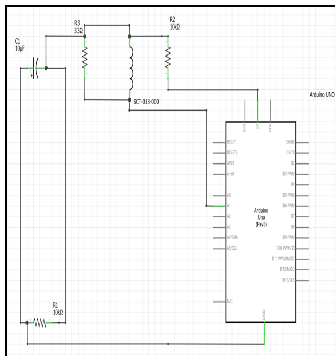
Fig -5: Circuit connections of current sensor
