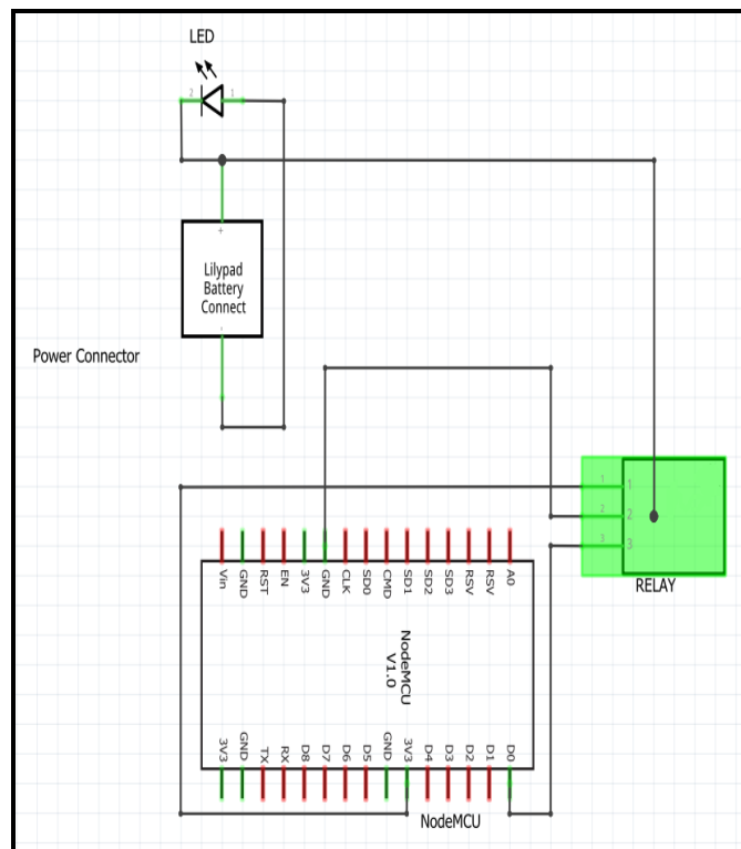
Fig -6: Circuit connections for powering off devices remotely
