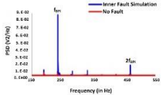
Fig.5(b). Characteristic Frequencies in the Spectral Analysis of Vibration of Induction Motor with Inner Race Bearing Fault
