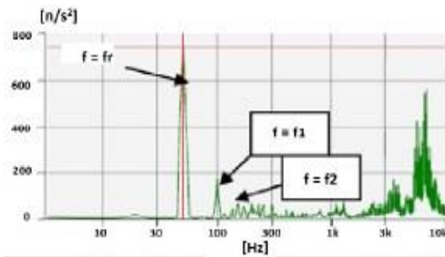
Fig. 4(b). Harmonic Vibration Spectra of Induction Motor with Bad Bearing
