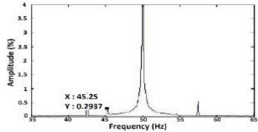
Fig. 8(a) FFT with initial condition for broken bars
