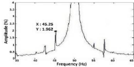
Fig. 8 ( b) FFT with 3 broken bars
