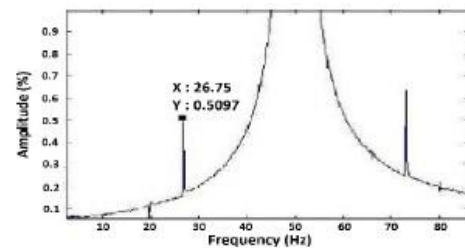
Fig. 9 (a) FFT with initial condition of Rotor's eccentricity
