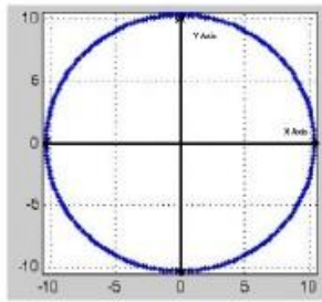
Fig.6(a). Motor Current's Park's Vector Representation at Healthy Case
