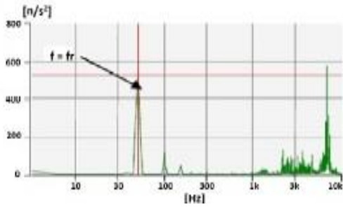
Fig. 4(a). Harmonic Vibration Spectra of Induction Motor with Good Bearing
