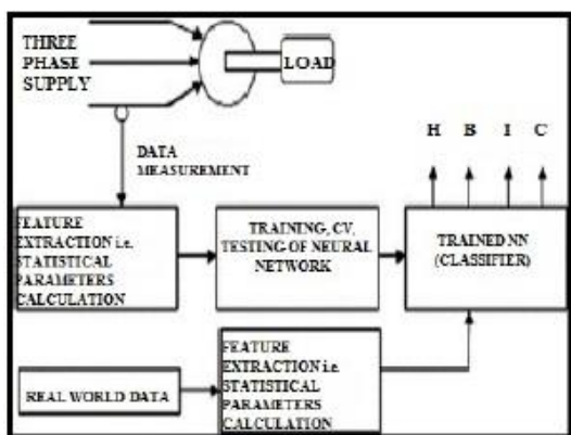
Fig. 10 Neural Network Schematic for Condition Monitoring of Induction Motor
