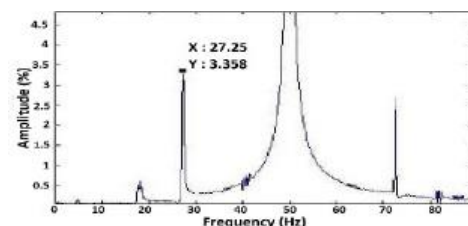
Fig. 9 (b) FFT with 87.3% of Rotor's eccentricity
