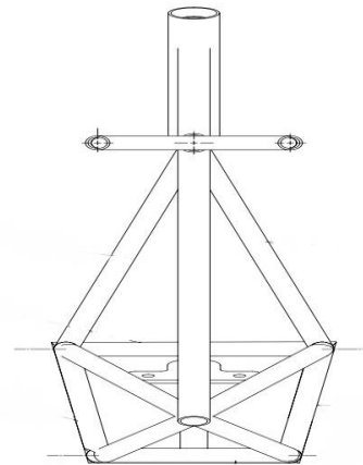
Fig -2: Front View Design of Steering Mechanism
