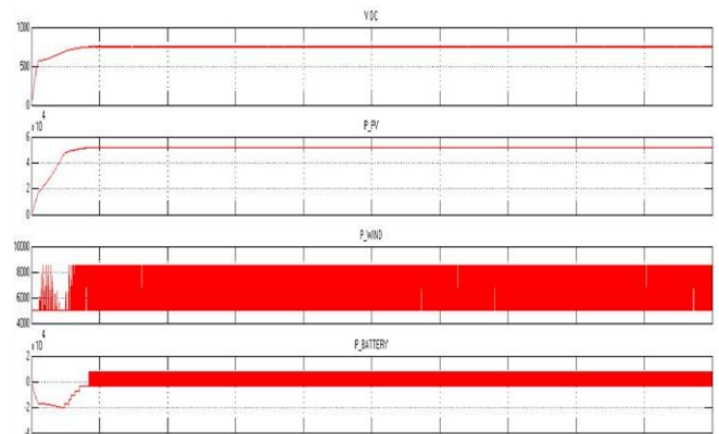
Fig.8 : Power at insolation 1000 w/m2, load : 40 KW
