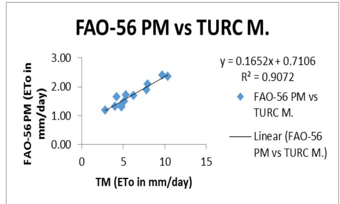
Chart 1 FAO-56 Penman Monteith Method and Turc Method
