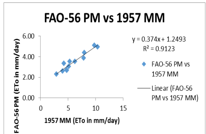
Chart 2 FAO-56 Penman Monteith Method and Makkink Method
