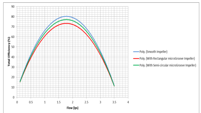
Chart-2. Performance graph of Flow vs Total Efficiency
