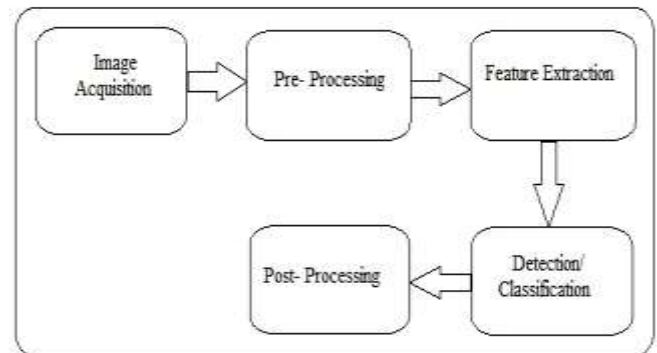
Fig -2: Automated fabric inspection system
