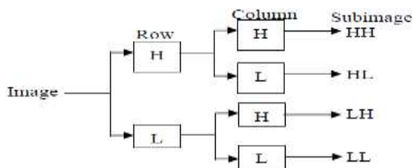
Fig -3: Tree Wavelet Decomposition of an image into four sub images
