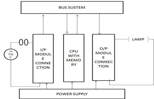
FIG- block diagram of plc system.
