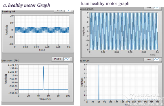
Figure No.1.9 Bearing Fault
