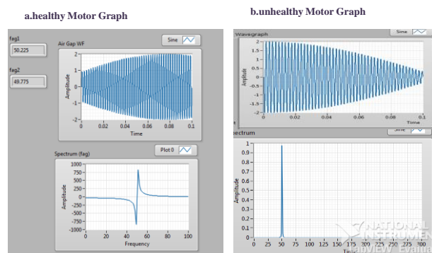
Figure No.1.8 Air Gap Eccentricity Fault
