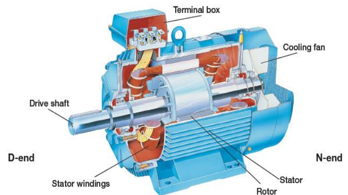
Figure No.1.1 Induction Motor Cut Way view
