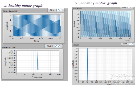
Figure no.1.10 Short Turn Faults
