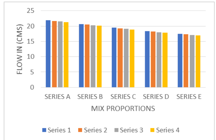
Figure 5.2 Flowability of different blends
