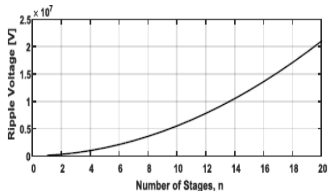
Fig 2. Variation of Ripple Voltage with number of stages in Cockcroft Walton.
