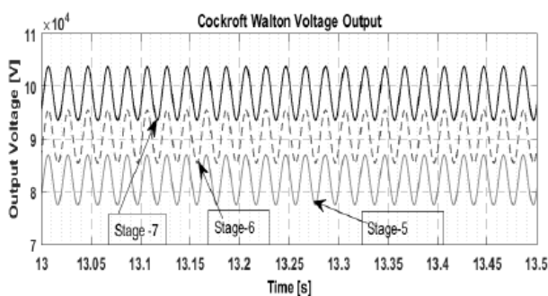
Fig. 7 Ripple Voltage Level of Output Stages
