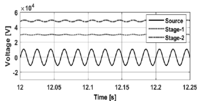
Fig. 5 Voltages of Source and Stage-1, 2
