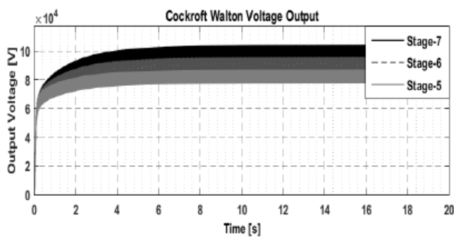
Fig. 6 Output of Final Three Stages
