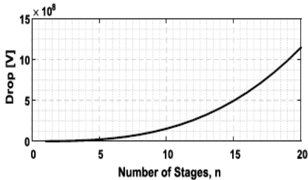
Fig. 3 Variation of Drop Voltage for a fixed frequency
