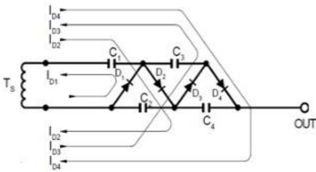
Fig -1: Cockcroft-Walton multiplier
