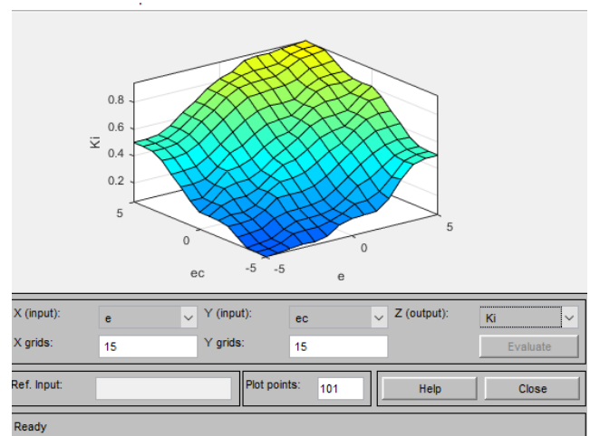
Figure 6: Surface Rule for Ki
