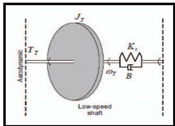
Figure 2: Mechanical model of drive train
