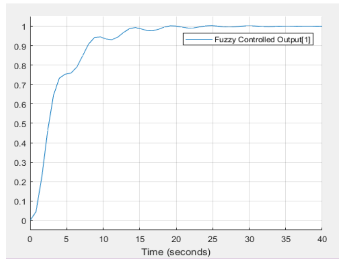
Figure 15: The unit step response of wind turbine with Fuzzy controller
