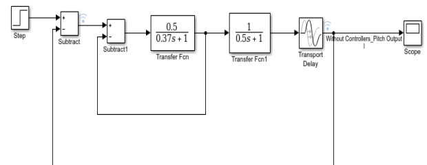
Figure 12: Wind Turbine System Without Controllers
