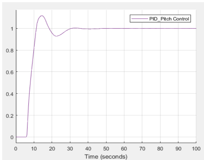
Figure 14: The unit step response of wind turbine with PID controller
