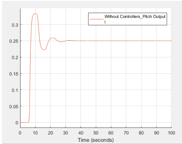
Figure 13: The unit step response of wind turbine without controllers
