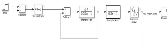
Figure 3: Simulink diagram of PID Controller Implementation
