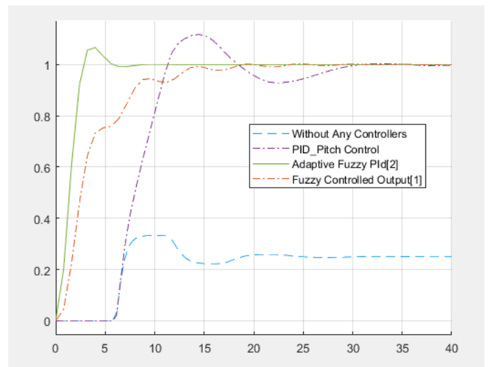
Figure 16: Comparison of unit step response of wind turbine pitch controllers
