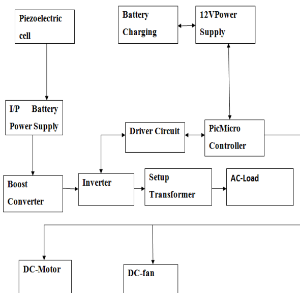
Fig -3: Working Of Foot Step Power Generation System
