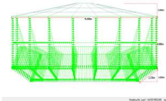
Figure-2: Hydrostatic load acted on Water Tank
