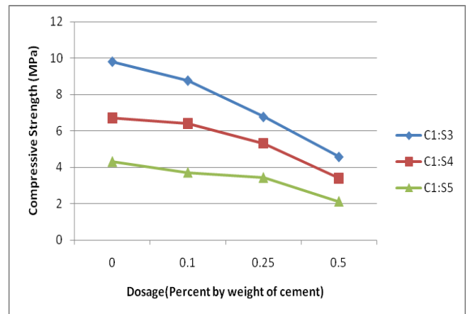
Fig. 4 Effect of Molasses on 7-days Compressive Strength of mortar
