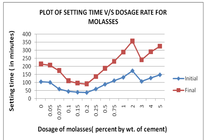
Fig. 1 Plot of Setting Time v/s Dosage Rate for Molasses
