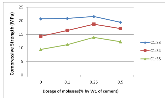
Fig. 5 Effect of Molasses on 28-days Compressive Strength of mortar
