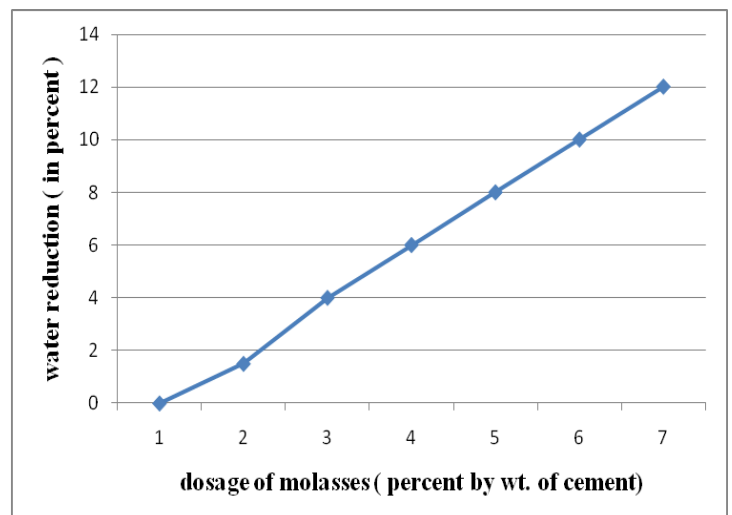
Fig. 2 Water Reduction Behaviour of Molasses in Mortar
