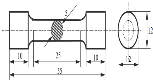
Fig (1) :The dimension of standard specimen for tensile test. (All dimensions are in mm)
