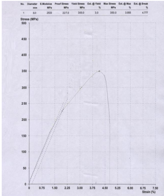
Fig(iii) : Stress-strain curve for Al6061 base alloy + 15% alumina and fly-ash
