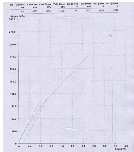
Fig(ii) : Stress-strain curve for Al6061 base alloy + 10% alumina and fly-ash
