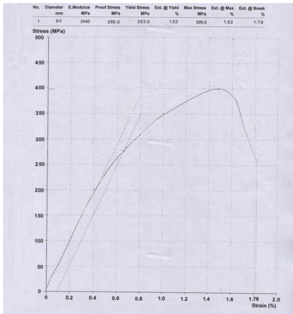
Fig(iv) : Stress-strain curve for Al6061 base alloy + 20% alumina and fly-ash
