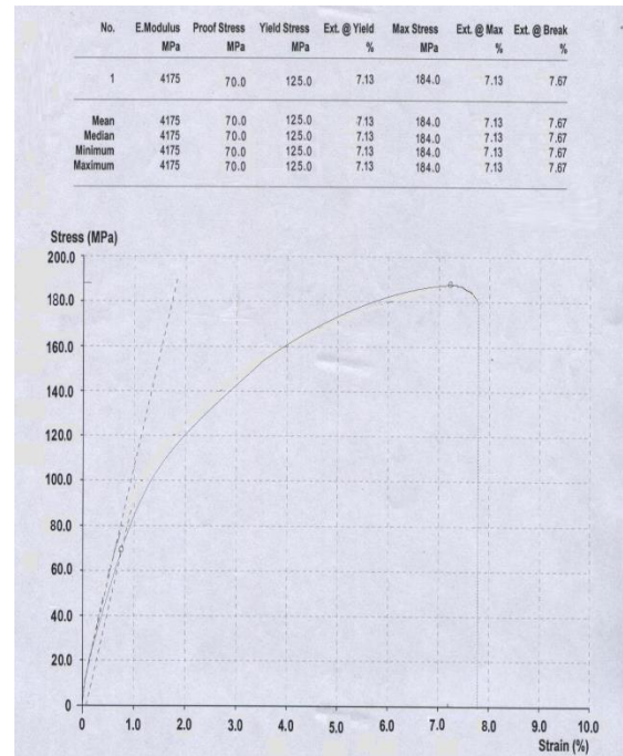
Fig (i) : Stress-strain curve for Al6061 base alloy
