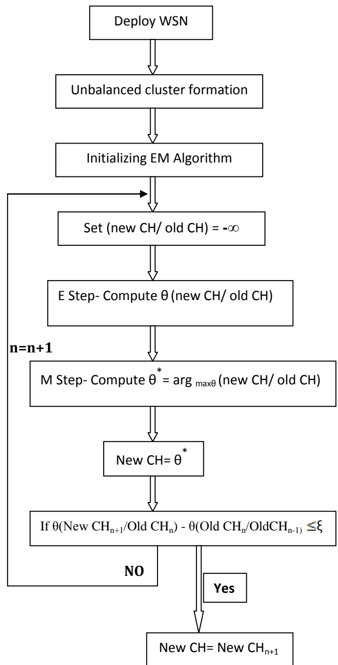
Fig 1. Flow diagram of algorithm
