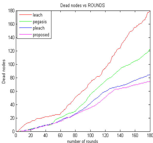
Chart 1-Number of dead nodes
