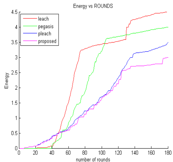
Chart 2- Energy consumption per round
