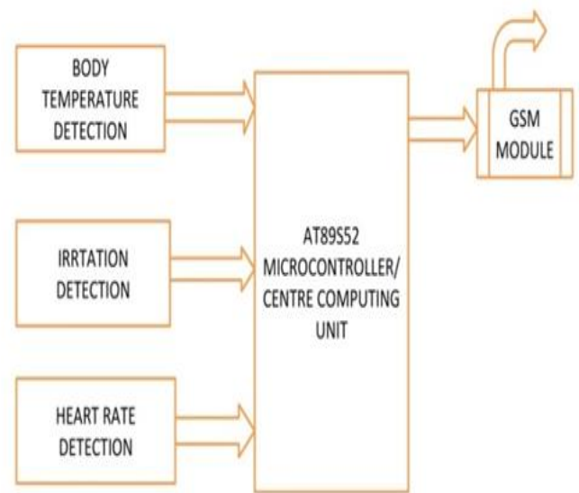
Fig.4 Architecture of a device.
