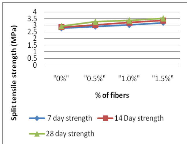
Chart -2: Split Tensile Strength results
