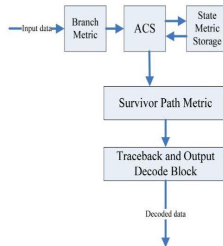
Figure 2: Block diagram of Viterbi decoder
