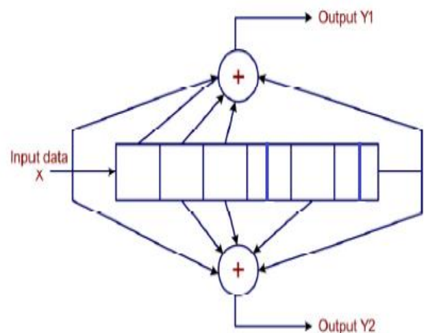
Figure 1: Convolutional encoder with constraint length k=9 and code rate (k/n)=1/2
