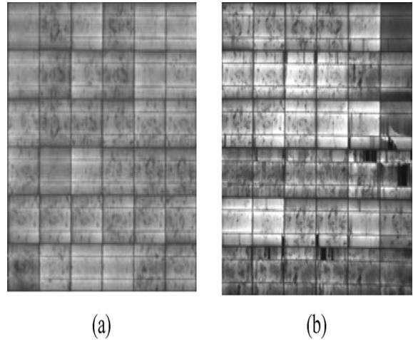
Fig. 2 EL images of (a) defect-free solar module, and (b) defective solar module.
