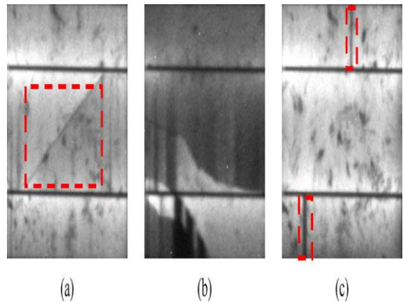
Fig. 3 Defect types of solar cells displayed in the EL image:
