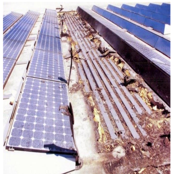
Fig 1.1(a) fire hazard in a 383 kW PV array in Bakersfield, California in 2009
