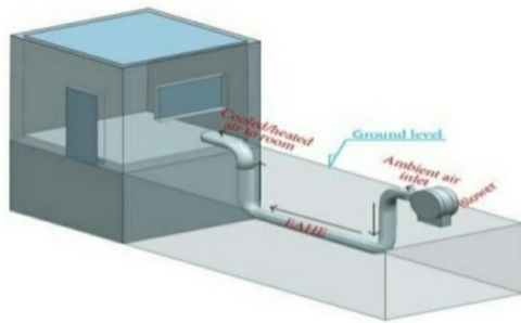
Fig 1.1 Open Loop System
