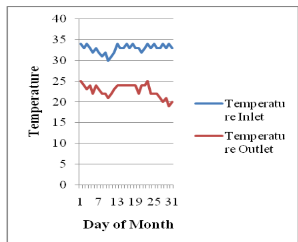
Fig. 3.2: Temperature at inlet and outlet and Max. Temp. Difference obtained on each day of a month
