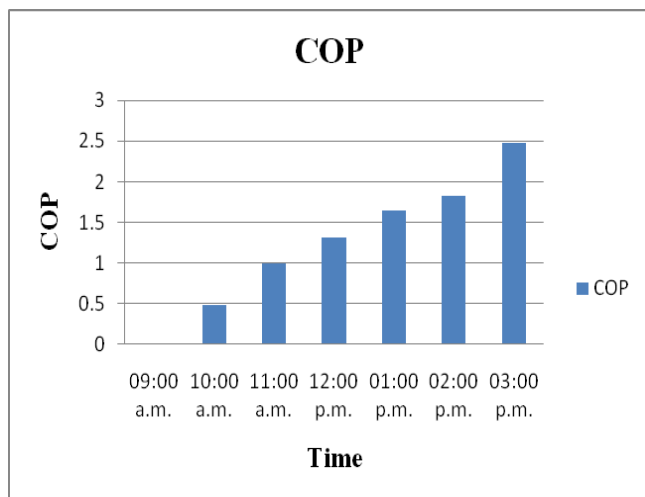
Chart -2 : Result for COP
