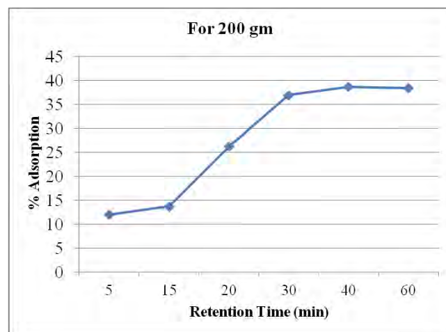
Chart 4: Effect of retention time on % adsorption of lead ion by 200 gm of orange peel
