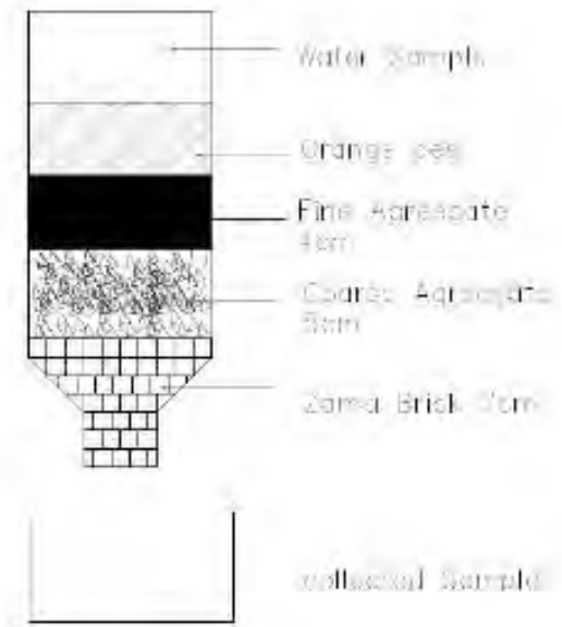
Fig 1: Experimental model of Column filter with orange peel
