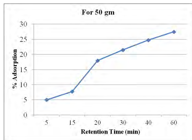
Chart 1: Effect of retention time on % adsorption of lead ion by 50 gm of orange peel
