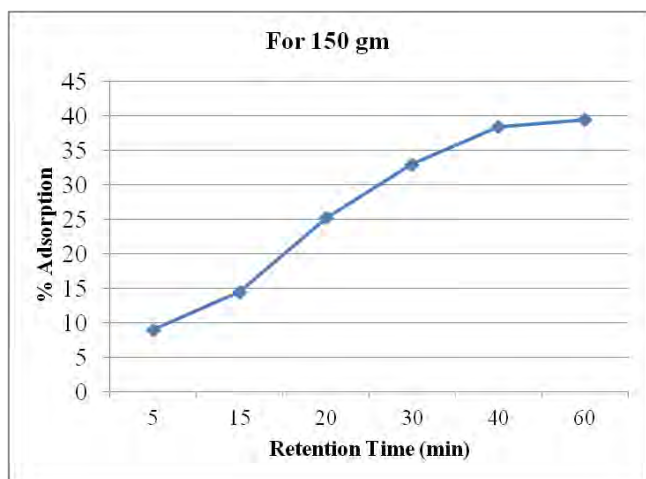
Chart 3: Effect of retention time on % adsorption of lead ion by 150 gm of orange peel
