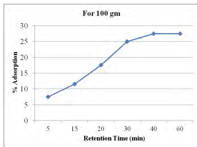
Chart 2: Effect of retention time on % adsorption of lead ion by 100 gm of orange peel
